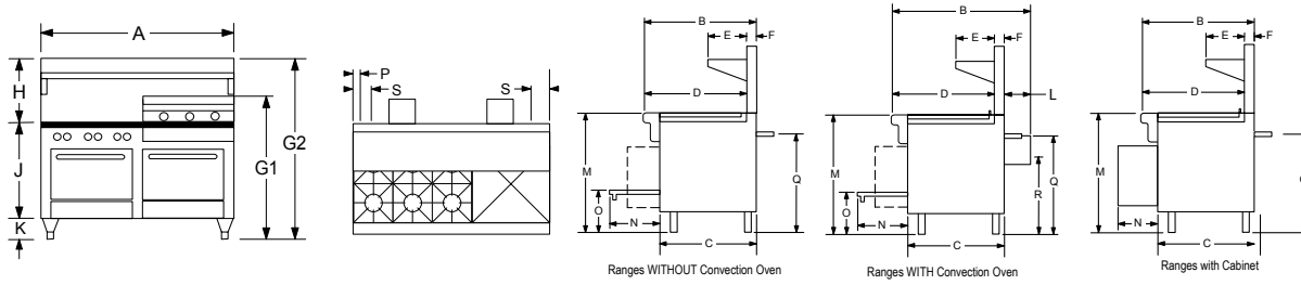
Dimensions - in(mm)
