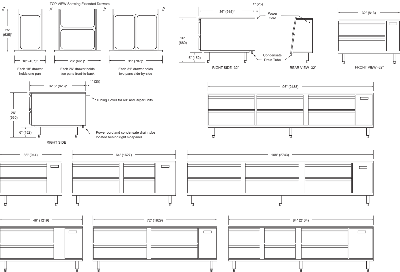
The drawer-front width, drawer-extension distance, and overall depth may vary (the maximum values are specified and shown)
