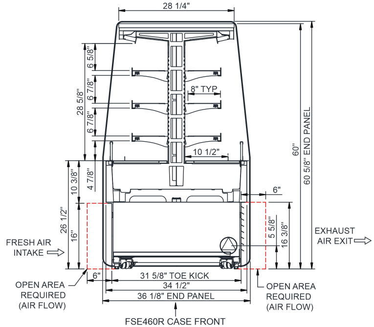
SIDE VIEW
