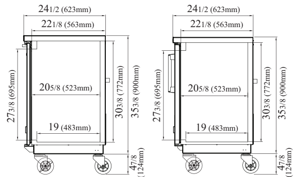
TBB-24-48SBD-N6 & TBB-24-48SGD-N SIDE VIEW
