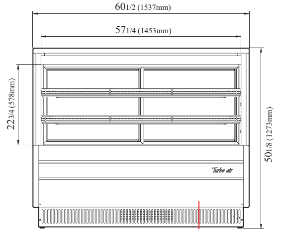
FRONT VIEW Power Cord (Back of the product)
