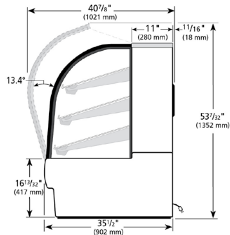
RIGHT VIEW
