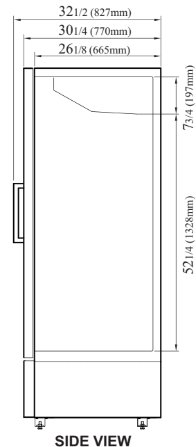
SIDE VIEW
