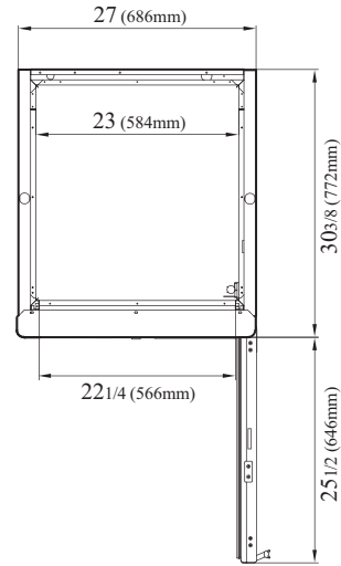
PLAN VIEW
