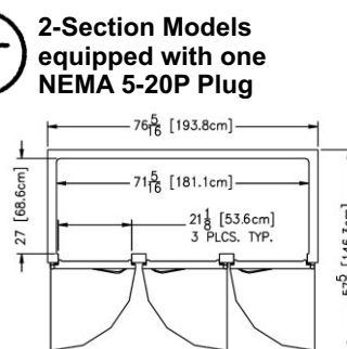
Plan - Three-Section
