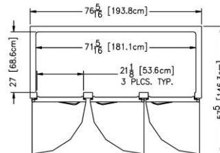
Plan - Three-Section
