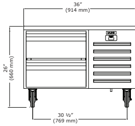
Front (CRB536)
