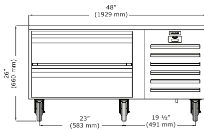
Front (CRB560)
