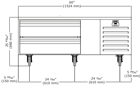
Front (CRB572)
