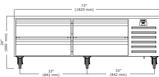
Front (CRB572)
