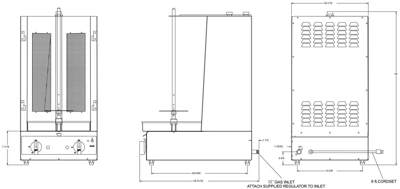
GAS MODEL SHOWN- ELECTRIC MODEL IS SIMILAR SIZE WITH A DIFFERENT CORDSET, HEATING ELEMENTS AND CONTROL PANEL. READ OWNERS MANUAL FOR PROPER INSTALLATION. THIS APPLIANCE SHOULD BE USED WITH ADEQUATE VENTILATION UNDER A HOOD.
