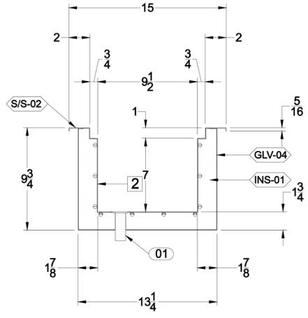
SECTION VIEW 1" = 1'-0"
