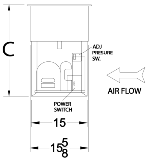
ELEVATION "A" 3/4" = 1'-0"
