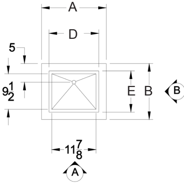
PLAN VIEW 3/4" = 1'-0"
