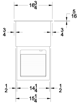
ELEVATION "B" 3/4" = 1'-0"
