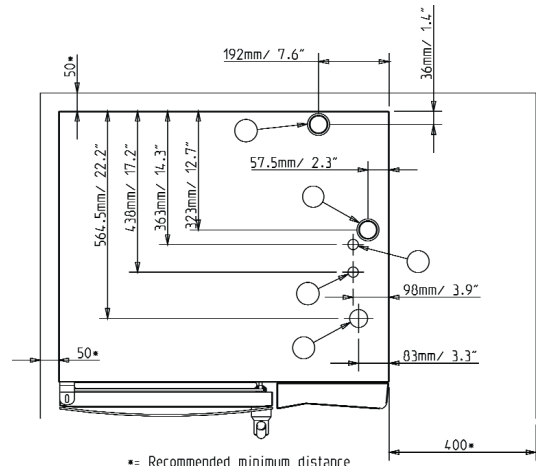
[Top View/Plan]
