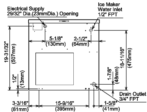
AIR-COOLED UNIT
