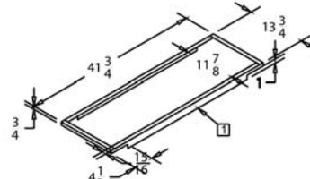
ADAPTER BAR (2) REQ'D
