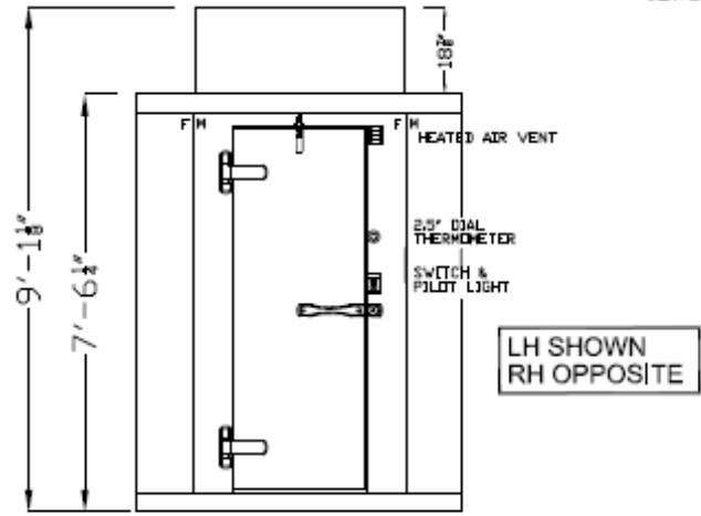
DOOR ELEVATION 46x7DS 26x7B DR P-P-FRZ STD THRESHOLD DETAIL 02
