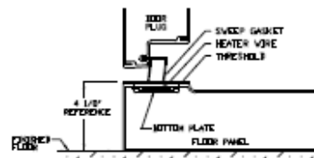
STANDARD WITH FLOOR FREEZER DETAIL 02
