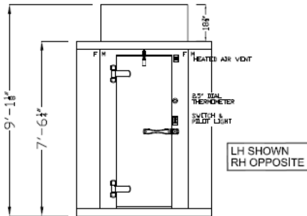
DOOR ELEVATION 46x7DS 26x7B DR P-P-FRZ STD THRESHOLD DETAIL 02
