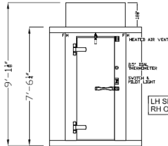
DOOR ELEVATION 46x78 26x78 DR P-P-FRZ STD THRESHOLD DETAIL 02
