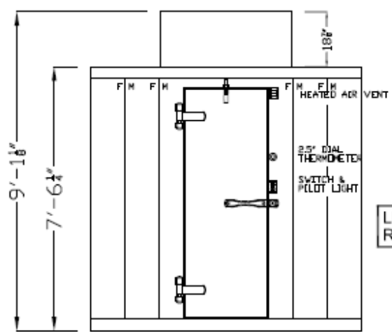
DOOR ELEVATION 46x82.25DS 26x78 DR STD FRZ STD THRESHOLD DETAIL 02
