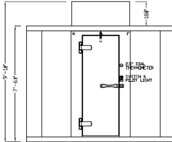
DOOR ELEVATION 46x82.25DS 26x78 DR P-P-CLR STD THRESHOLD DETAIL 01
