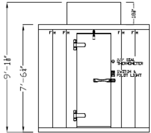
DOOR ELEVATION 46x82.25DS 26x78 DR P-P-CLR STD THRESHOLD DETAIL 01
