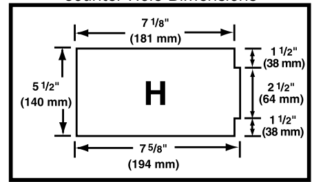
Counter Hole Dimensions
