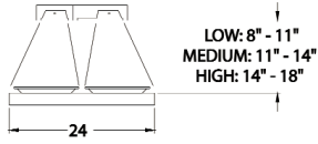
MOUNTING HEIGHT FROM NON-COMBUSTIBLE SURFACE
